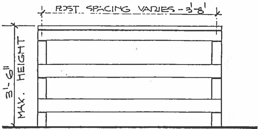
THREE-RAIL
